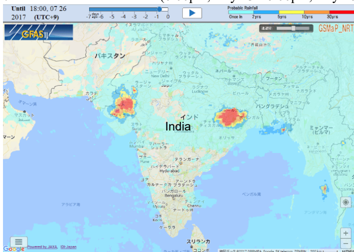
72 Hours Probable Rainfall (6:00pm, July 23 - 6:00pm, July 26 JST)
