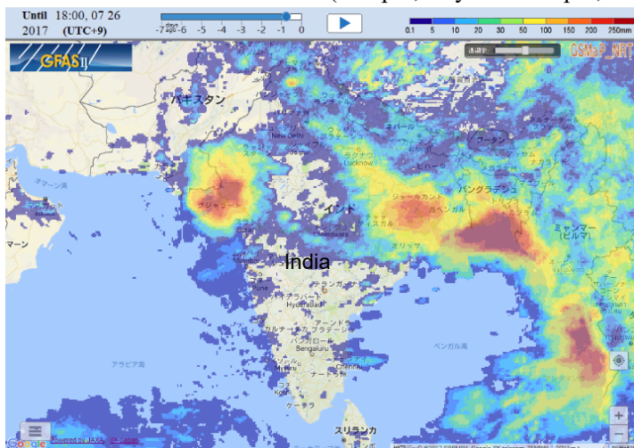
72 Hours Accumulated Rainfall (6:00pm, July 23 - 6:00pm, July 26 JST)
