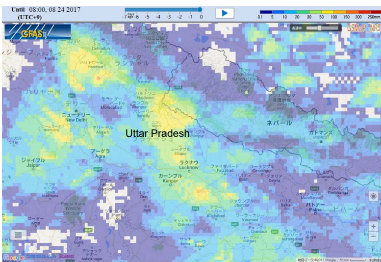
72 Hours Accumulated Rainfall (8:00am, August 21 - 8:00am, August 24 JST)
