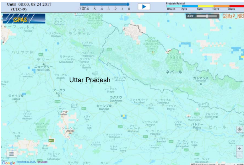
72 Hours Probable Rainfall (8:00am, August 21 - 8:00am, August 24 JST)
